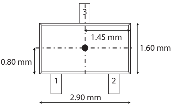
13.2 SOT Package
